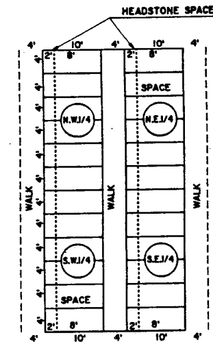
TYPICAL BLOCK LAYOUT BLOCKS 705 TO 863
